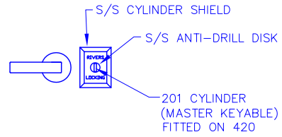
OUTSIDE VIEW (SERIES 420 ONLY)
